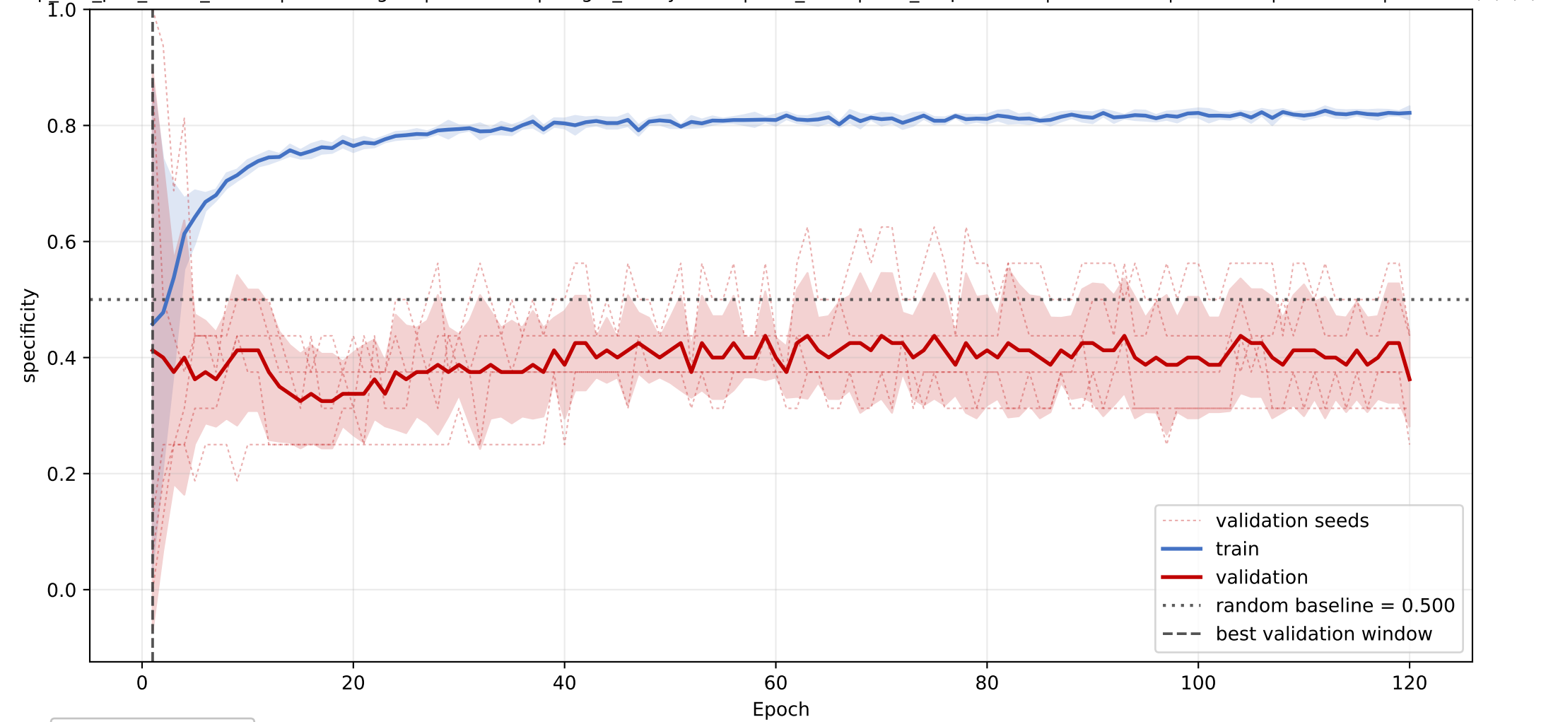
PS+PGP+DAG+TAG: mean specificity learning curve across seeds
