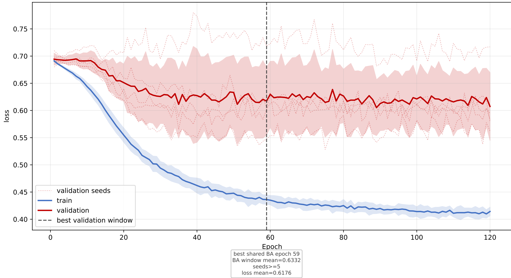
LPC+LPE+LPG: mean loss learning curve across seeds
