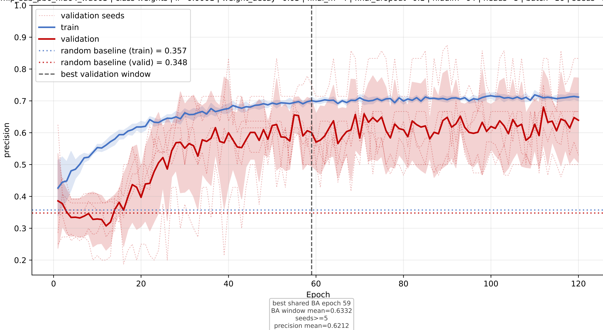
LPC+LPE+LPG: mean precision learning curve across seeds
