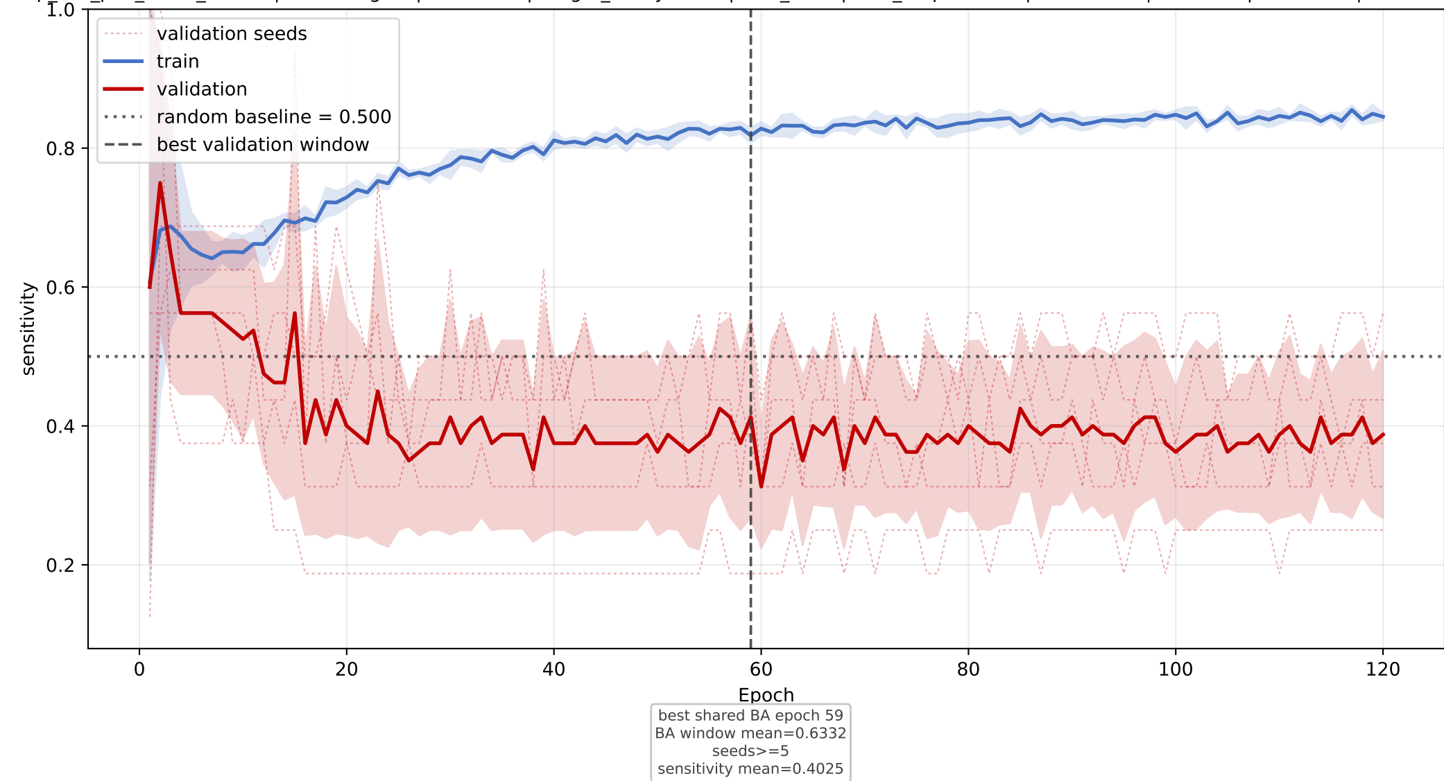
LPC+LPE+LPG: mean sensitivity learning curve across seeds
