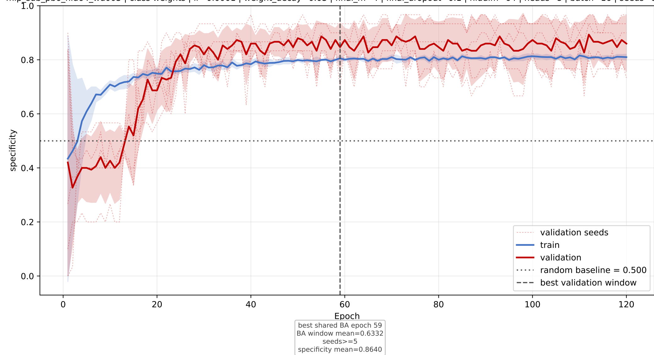
LPC+LPE+LPG: mean specificity learning curve across seeds
