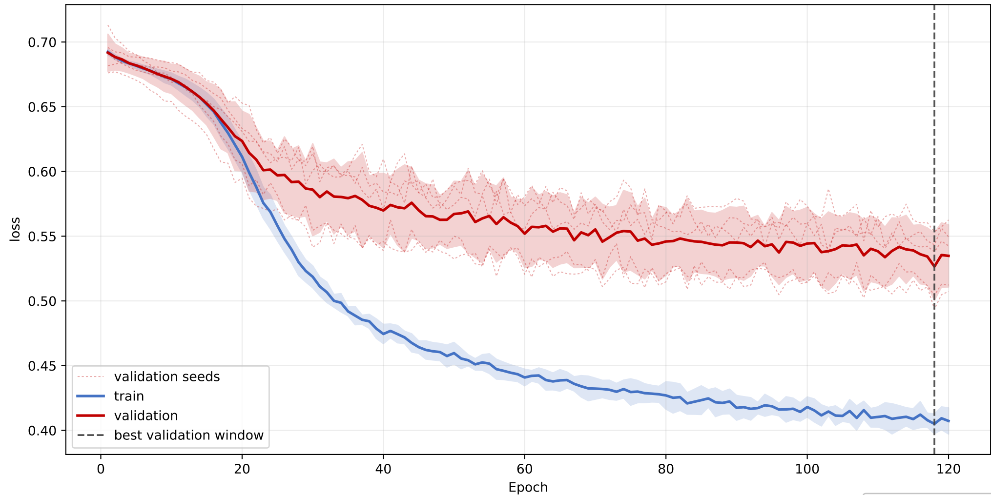
PG: mean loss learning curve across seeds
