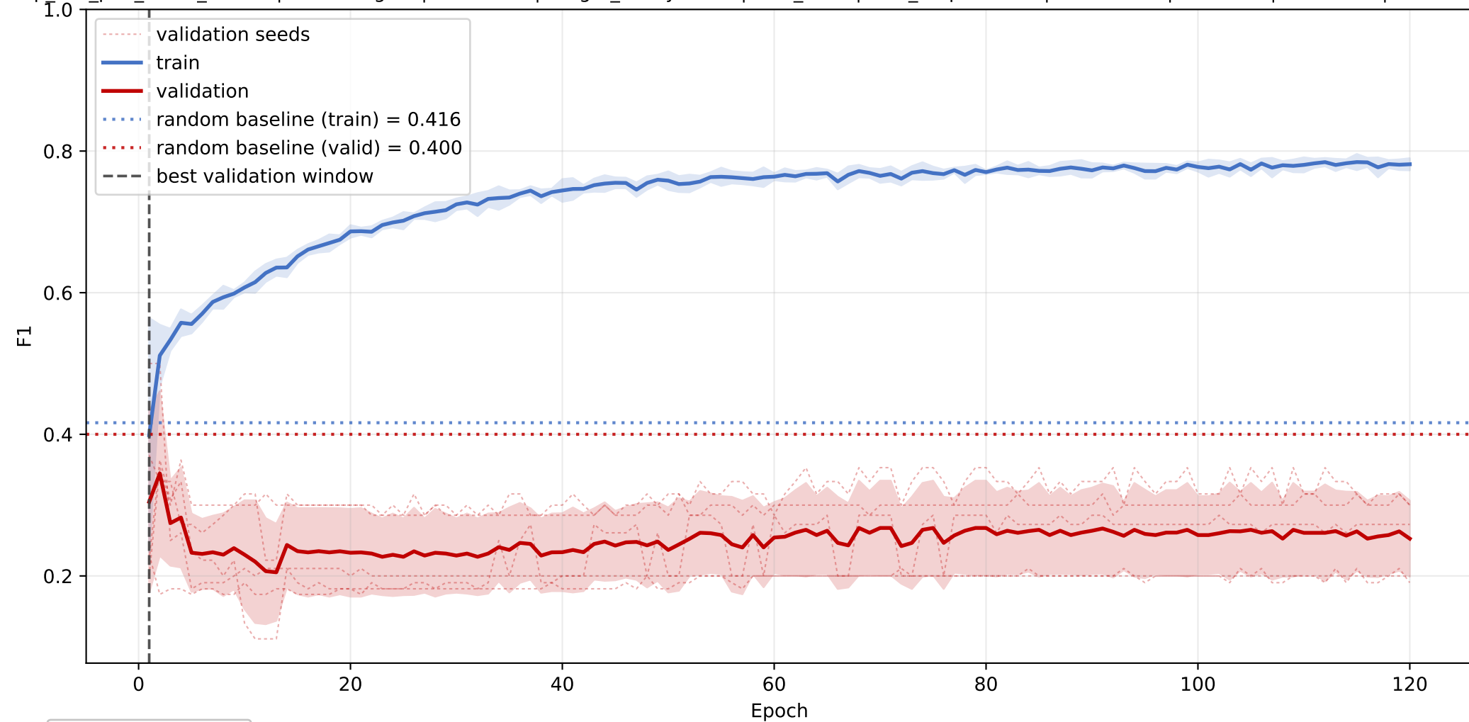
PS+PGP+DAG+TAG: mean F1 learning curve across seeds
