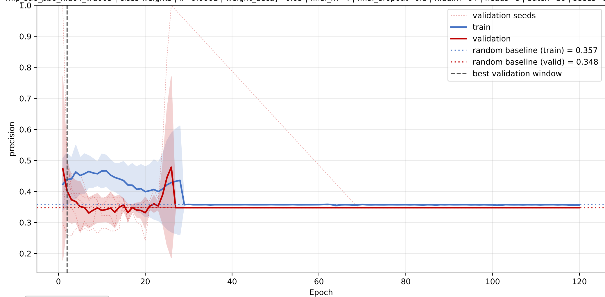
LPC+LPE+LPG: mean precision learning curve across seeds
