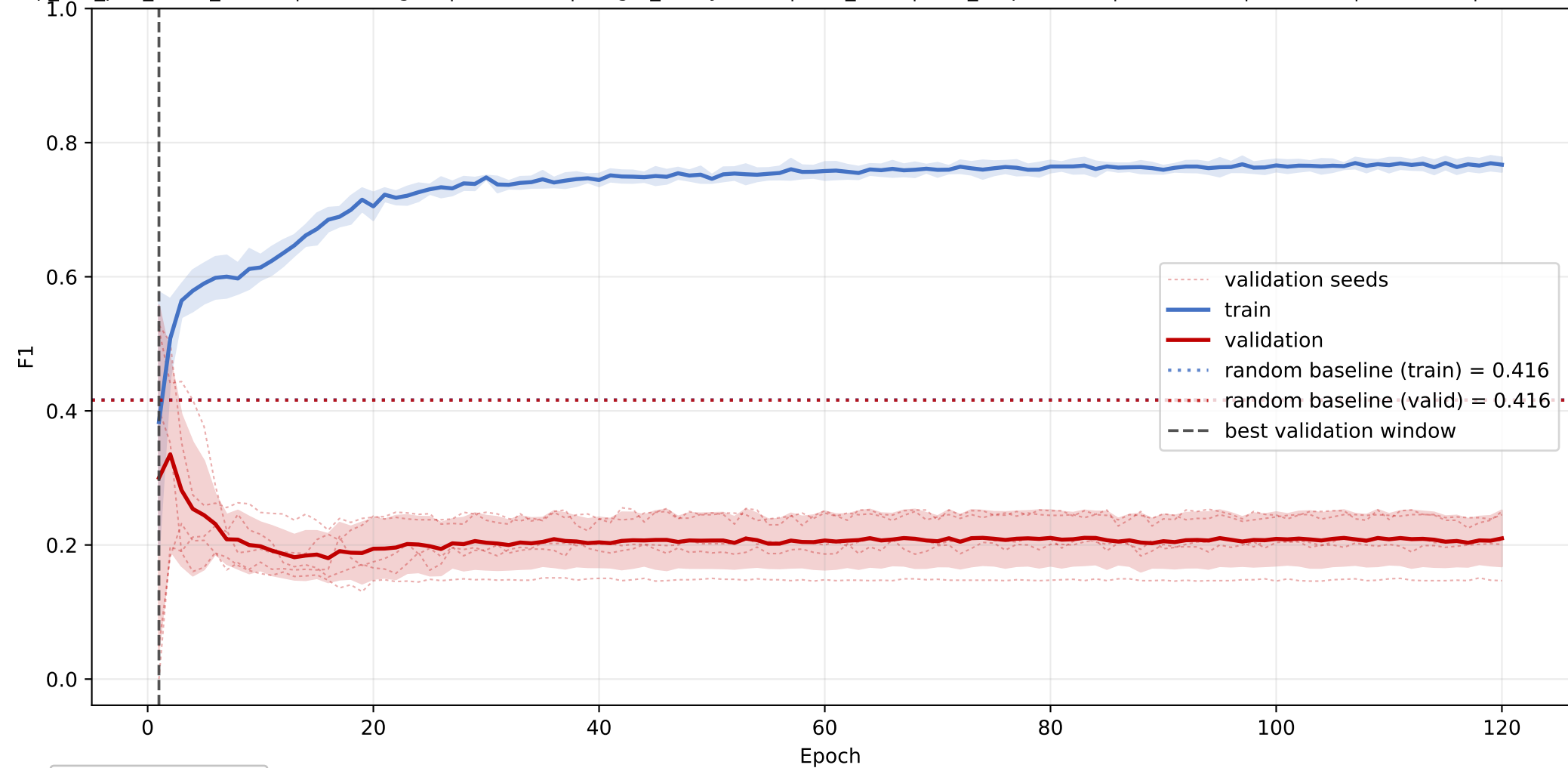
PC: mean F1 learning curve across seeds
