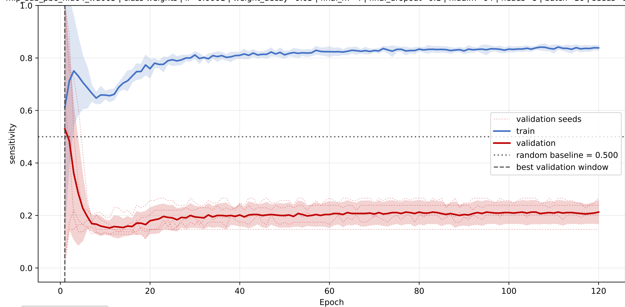
PC: mean sensitivity learning curve across seeds
