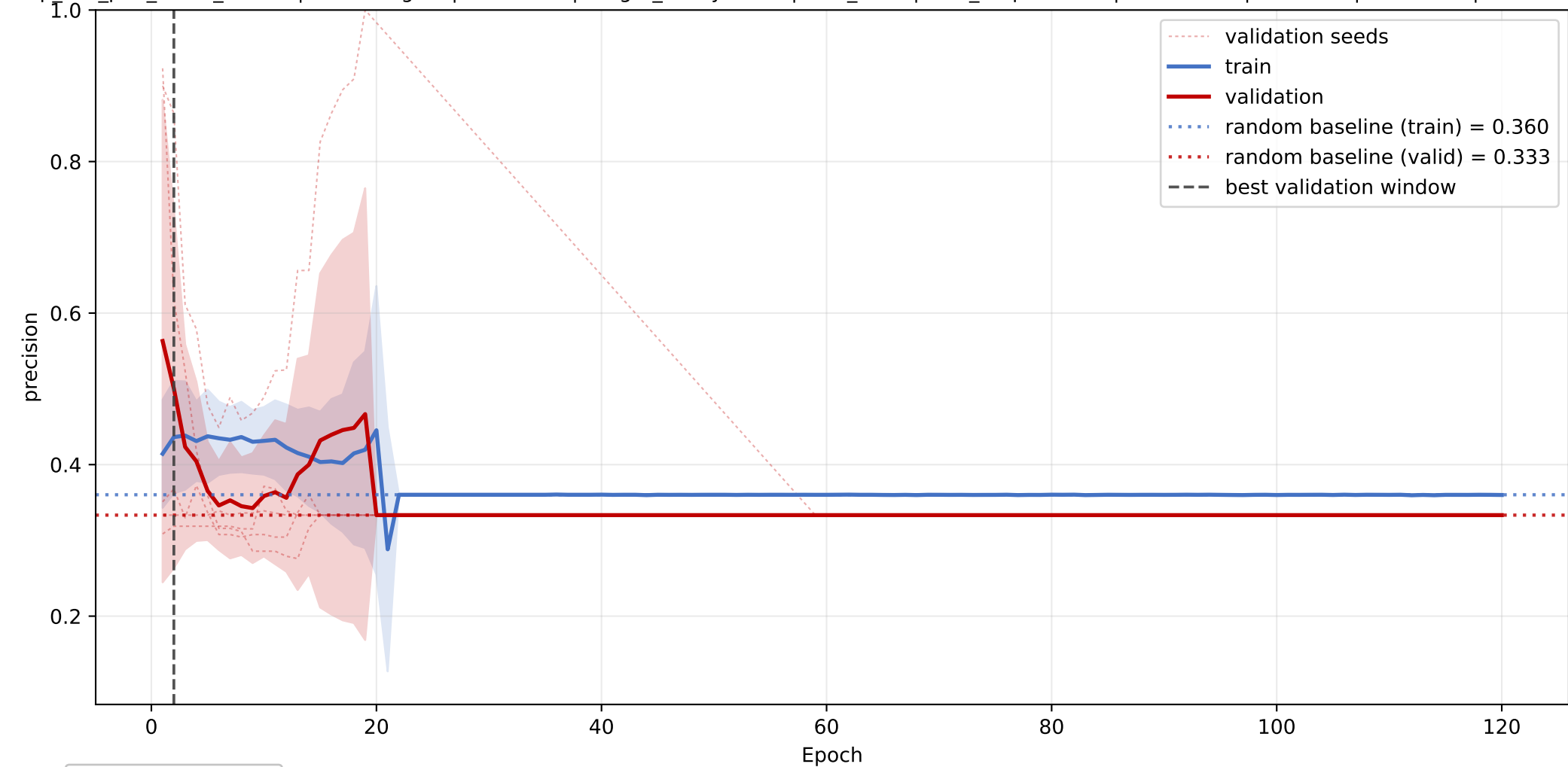
PE: mean precision learning curve across seeds
