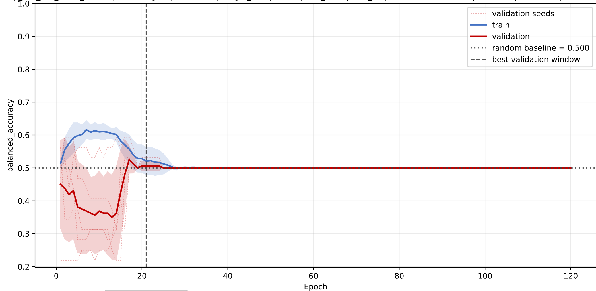
PS+PGP+DAG+TAG: mean balanced_accuracy learning curve across seeds
