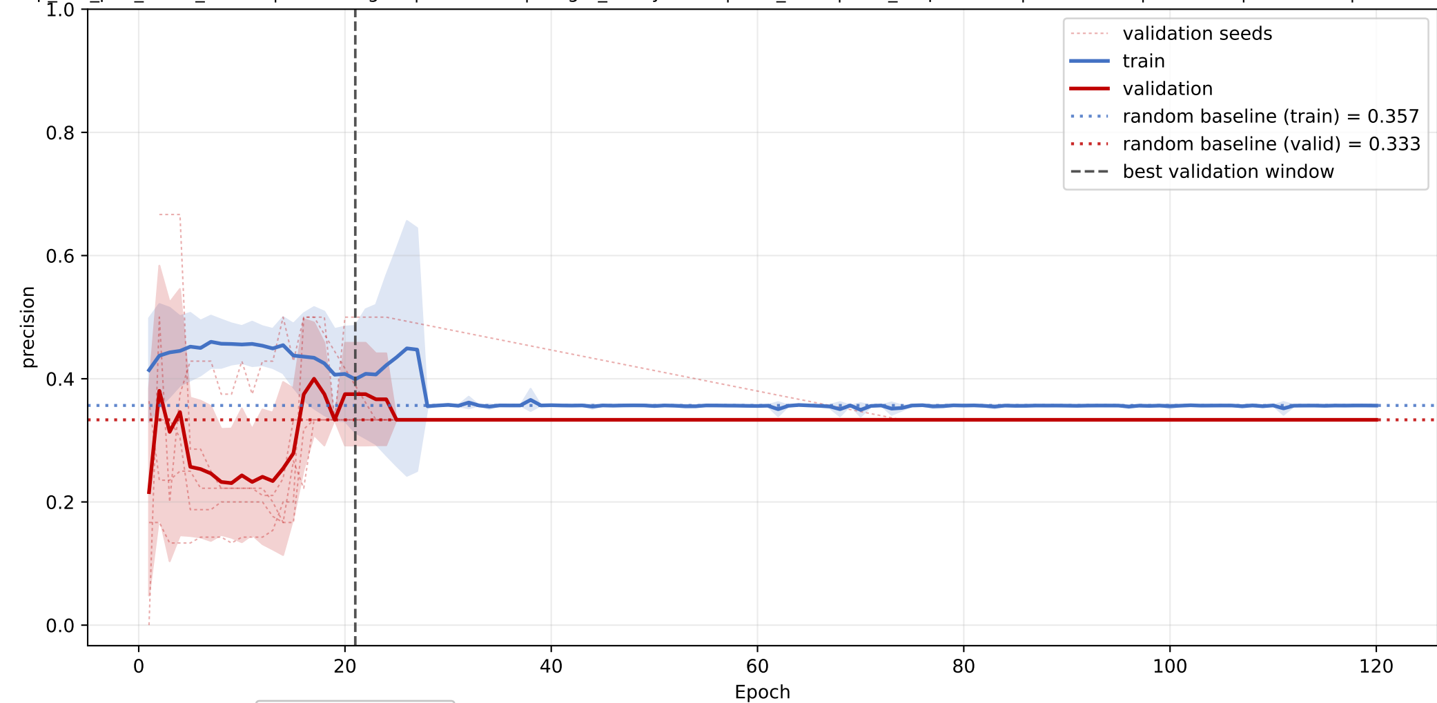
PS+PGP+DAG+TAG: mean precision learning curve across seeds
