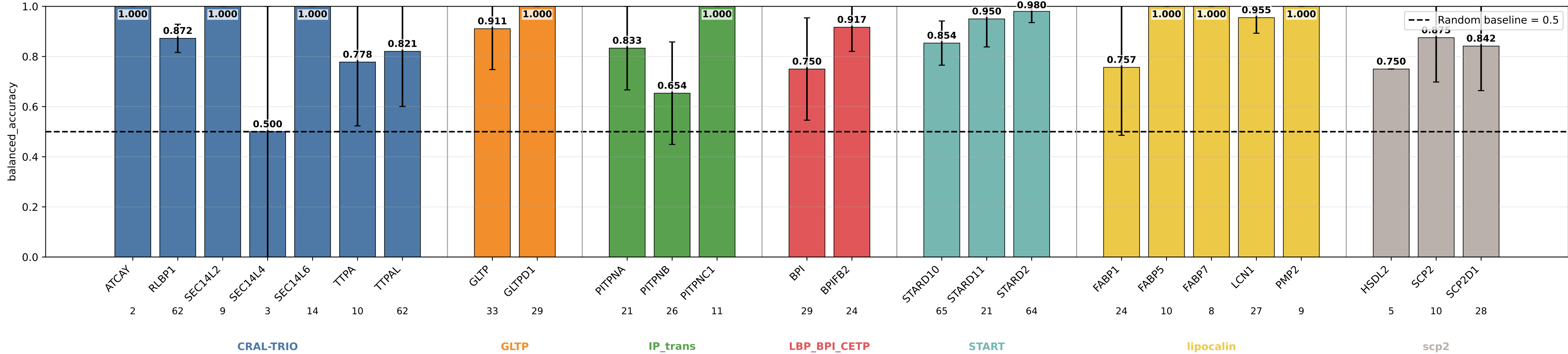
structural_pretrain_family_unfrozen_protunion14 balanced_accuracy by subgroup structural_pretrain_family_unfrozen_protunion14 | class weights | lr=0.0001 | weight_decay=0.001 | final_m=4 | final_dropout=0.1 | hiddim=64 | heads=8 | batch=16 | ep=120 | seeds=0,1,2,3,4
