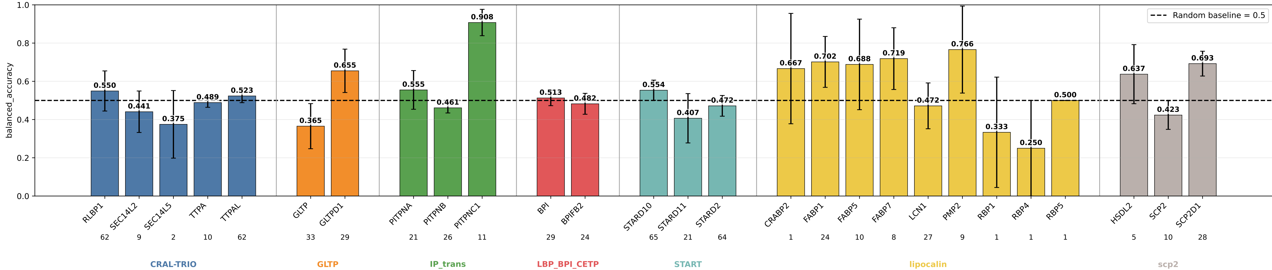
geometric_edge_attention_protgeom_family_neutral_normalized_bilinear_fusion_bilinear_norm_rim_ev28_lipid_class balanced_accuracy by subgroup geometric_edge_attention_protgeom_family_neutral_normalized_bilinear_fusion_bilinear_norm_rim_ev28_lipid_class | class weights | lr=0.0001 | weight_decay=0.01 | final_m=4 | final_dropout=0.1 | hiddim=8 | heads=8 | batch=16 | ep=120 | seeds=0,1,2,3,4
