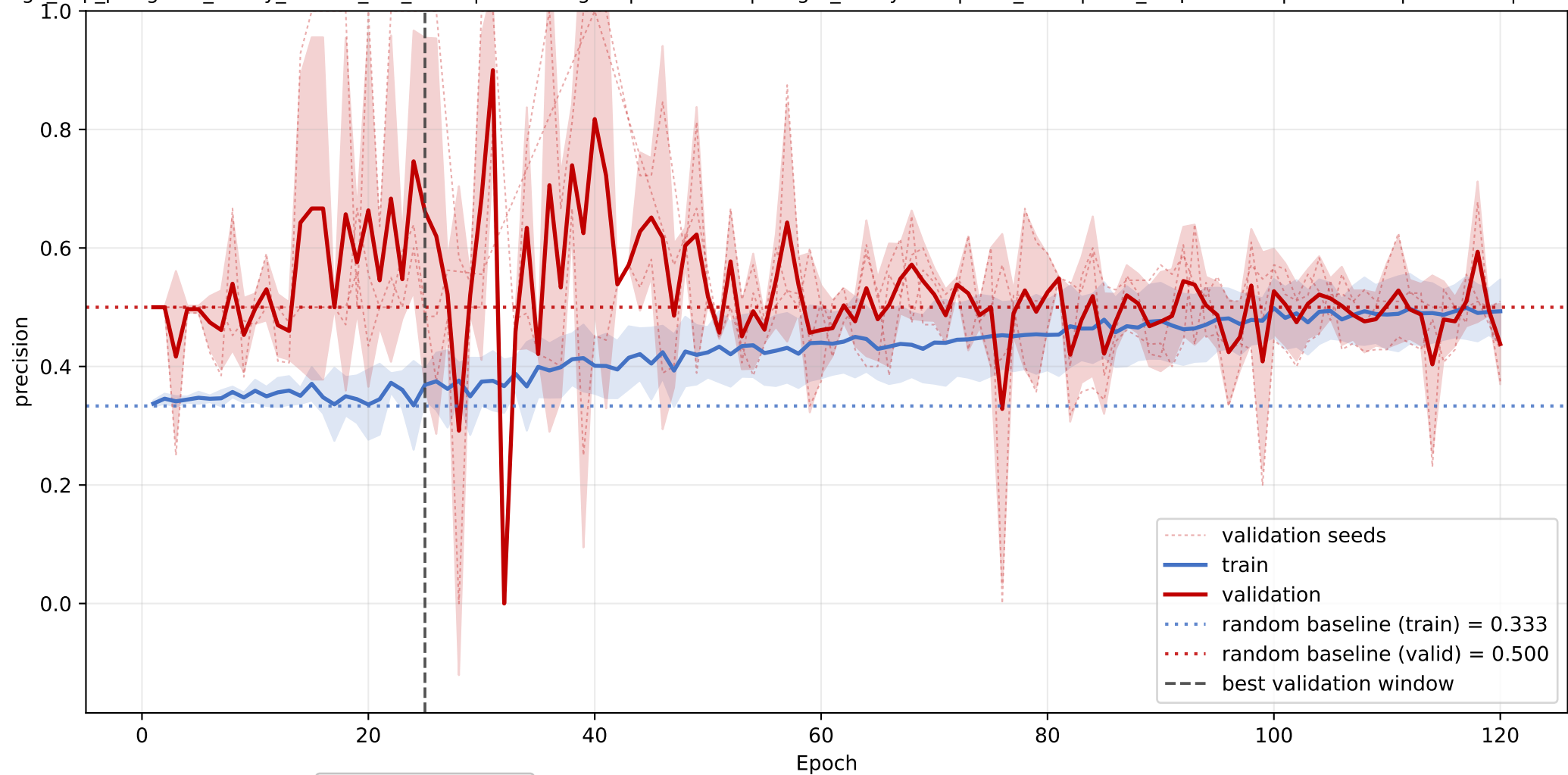
GLTP: mean precision learning curve across seeds
