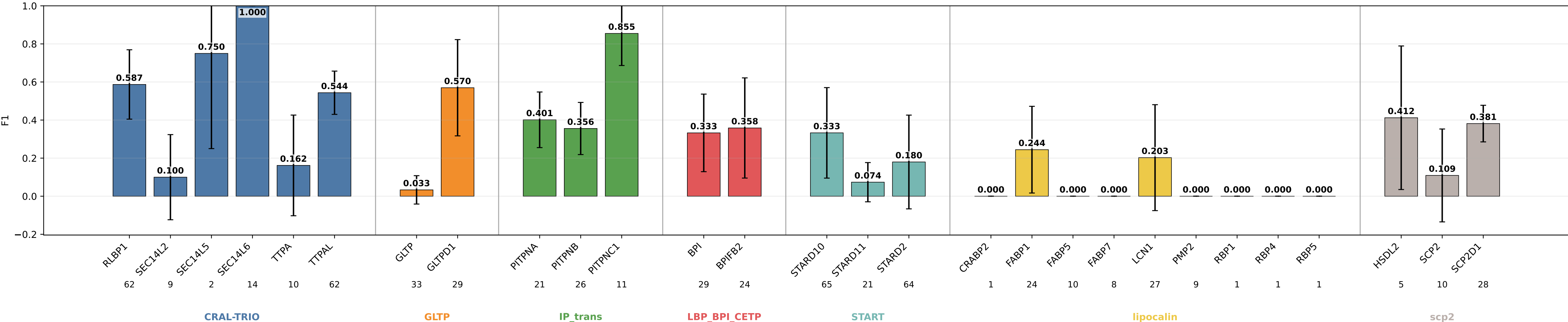
geometric_edge_mlp_protgeom_family_neutral_normalized_bilinear_fusion_bilinear_norm_attnbypocket F1 by subgroup geometric_edge_mlp_protgeom_family_neutral_normalized_bilinear_fusion_bilinear_norm_attnbypocket | class weights | lr=0.0001 | weight_decay=0.01 | final_m=4 | final_dropout=0.1 | hiddim=8 | heads=8 | batch=16 | ep=120 | seeds=0,1,2,3,4
