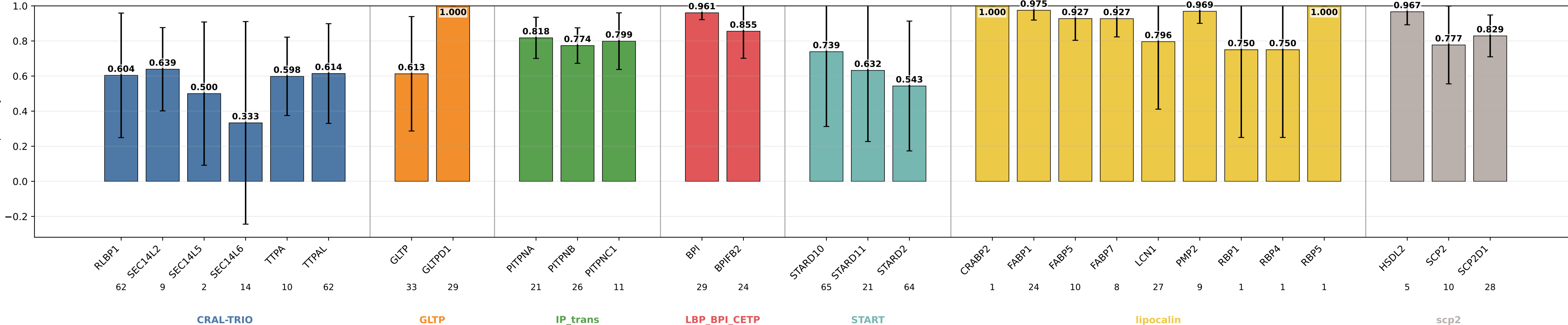
geometric_edge_mlp_protgeom_family_neutral_normalized_bilinear_fusion_bilinear_norm_attnpool_pocketbias specificity by subgroup geometric_edge_mlp_protgeom_family_neutral_normalized_bilinear_fusion_bilinear_norm_attnpool_pocketbias | class weights | lr=0.0001 | weight_decay=0.01 | final_m=4 | final_dropout=0.1 | hiddim=8 | heads=8 | batch=16 | ep=120 | seeds=0,1,2,3,4
