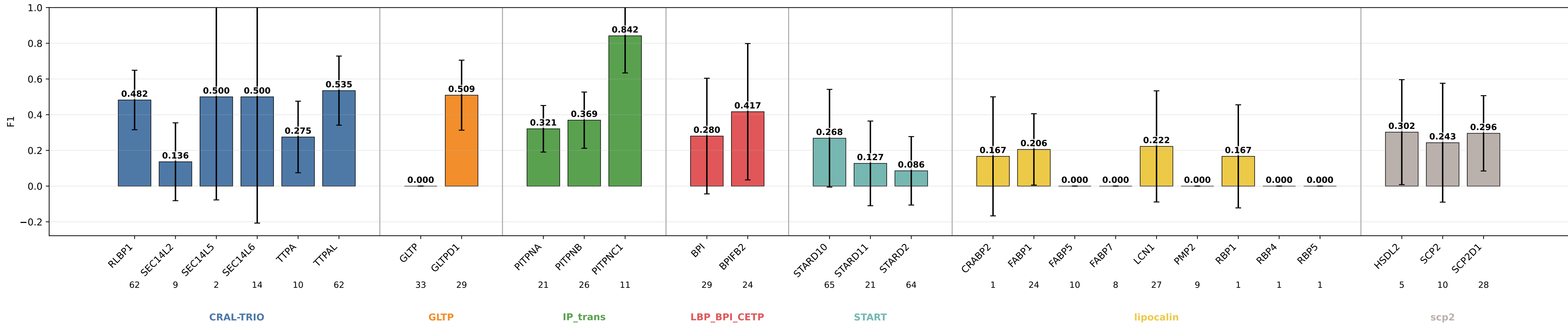
geometric_edge_mlp_protgeom_family_neutral_normalized_bilinear_fusion_bilinear_norm_ckpt30 F1 by subgroup geometric_edge_mlp_protgeom_family_neutral_normalized_bilinear_fusion_bilinear_norm_ckpt30 | class weights | lr=0.0001 | weight_decay=0.01 | final_m=4 | final_dropout=0.1 | hiddim=8 | heads=8 | batch=16 | ep=120 | seeds=0,1,2,3,4
