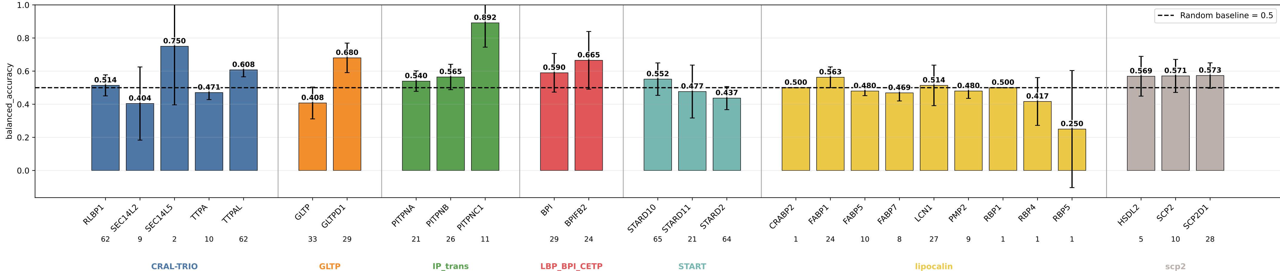
geometric_edge_mlp_protgeom_family_neutral_normalized_bilinear_fusion_bilinear_norm_ckpt30 balanced_accuracy by subgroup geometric_edge_mlp_protgeom_family_neutral_normalized_bilinear_fusion_bilinear_norm_ckpt30 | class weights | lr=0.0001 | weight_decay=0.01 | final_m=4 | final_dropout=0.1 | hiddim=8 | heads=8 | batch=16 | ep=120 | seeds=0,1,2,3,4
