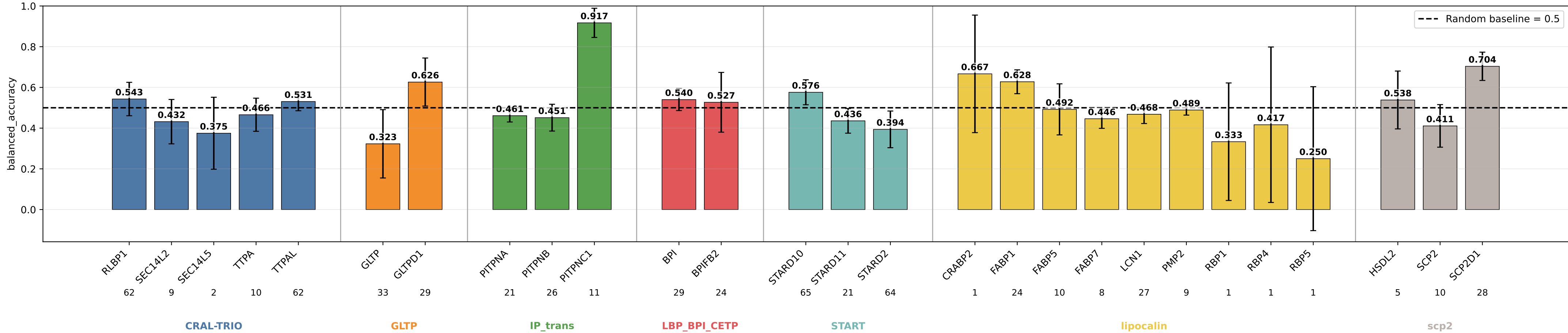
geometric_edge_mlp_protgeom_family_neutral_normalized_bilinear_fusion_bilinear_norm_lipid_class balanced_accuracy by subgroup geometric_edge_mlp_protgeom_family_neutral_normalized_bilinear_fusion_bilinear_norm_lipid_class | class weights | lr=0.0001 | weight_decay=0.01 | final_m=4 | final_dropout=0.1 | hiddim=8 | heads=8 | batch=16 | ep=120 | seeds=0,1,2,3,4
