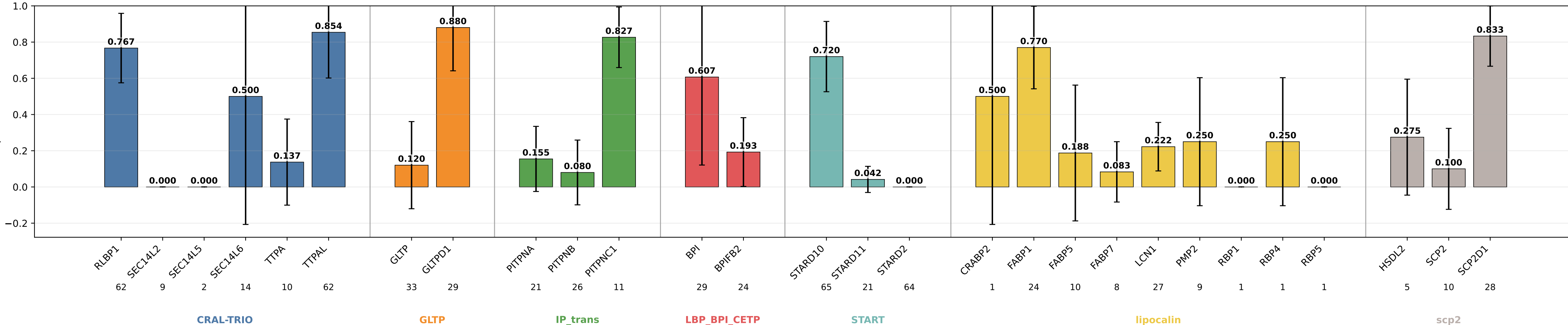
geometric_edge_mlp_protgeom_family_neutral_normalized_bilinear_fusion_bilinear_norm_lipid_class precision by subgroup geometric_edge_mlp_protgeom_family_neutral_normalized_bilinear_fusion_bilinear_norm_lipid_class | class weights | lr=0.0001 | weight_decay=0.01 | final_m=4 | final_dropout=0.1 | hiddim=8 | heads=8 | batch=16 | ep=120 | seeds=0,1,2,3,4
