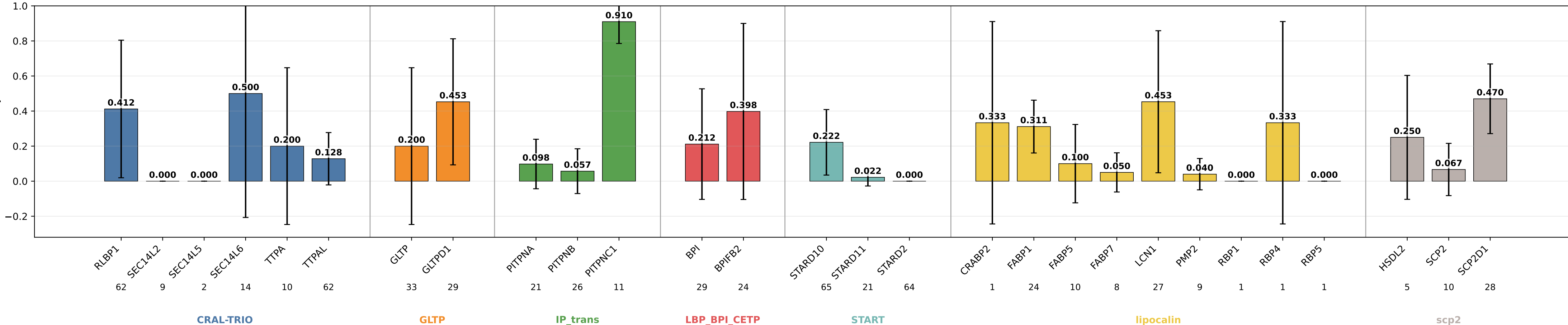
geometric_edge_mlp_protgeom_family_neutral_normalized_bilinear_fusion_bilinear_norm_lipid_class | class weights | lr=0.0001 | weight_decay=0.01 | final_m=4 | final_dropout=0.1 | hiddim=8 | heads=8 | batch=16 | ep=120 | seeds=0,1,2,3,4
