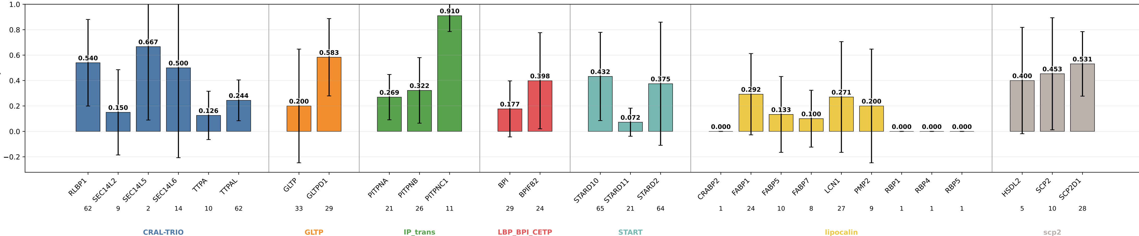
geometric_edge_mlp_protgeom_family_neutral_normalized_bilinear_fusion_bilinear_norm_pocketonly sensitivity by subgroup geometric_edge_mlp_protgeom_family_neutral_normalized_bilinear_fusion_bilinear_norm_pocketonly | class weights | lr=0.0001 | weight_decay=0.01 | final_m=4 | final_dropout=0.1 | hiddim=8 | heads=8 | batch=16 | ep=120 | seeds=0,1,2,3,4
