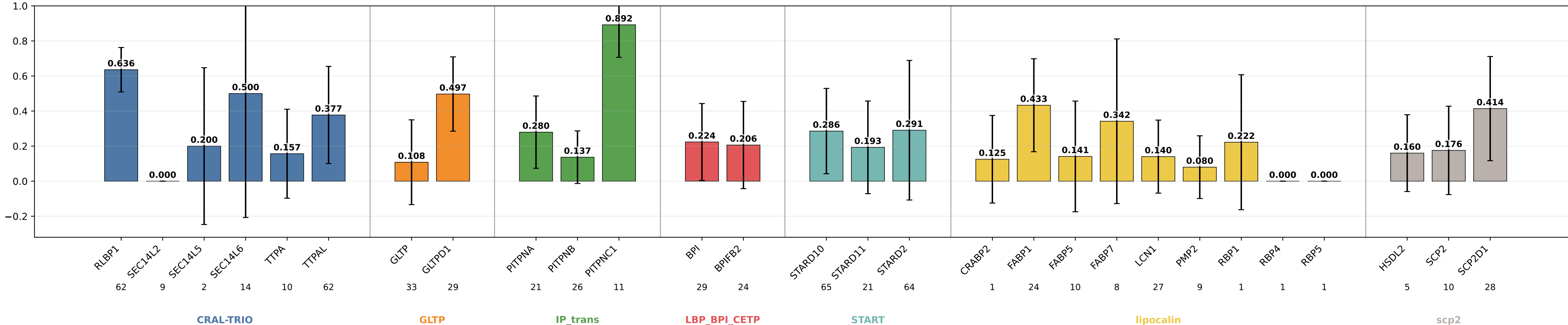
geometric_edge_mlp_protgeom_family_neutral_normalized_bilinear_fusion_bilinear_norm_rim_ev28 F1 by subgroup geometric_edge_mlp_protgeom_family_neutral_normalized_bilinear_fusion_bilinear_norm_rim_ev28 | class weights | lr=0.0001 | weight_decay=0.01 | final_m=4 | final_dropout=0.1 | hiddim=8 | heads=8 | batch=16 | ep=120 | seeds=0,1,2,3,4
