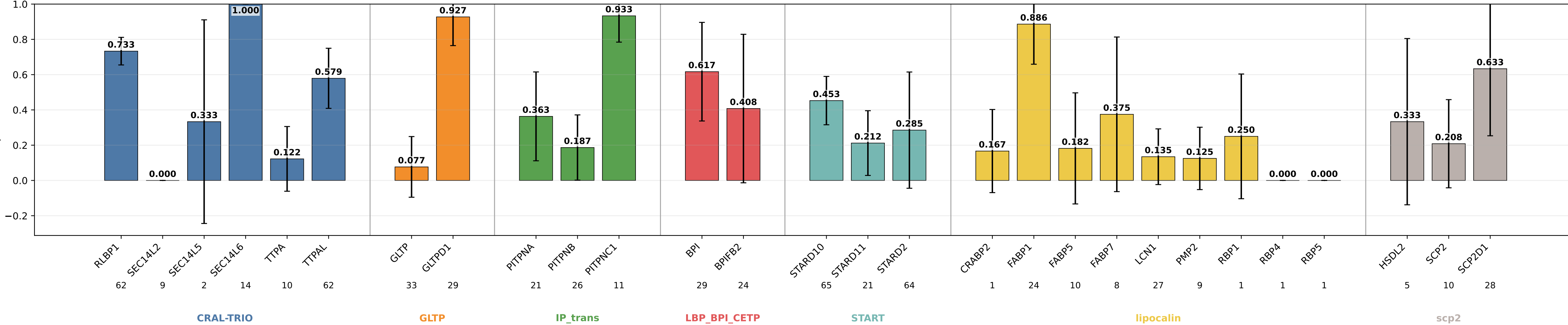
geometric_edge_mlp_protgeom_family_neutral_normalized_bilinear_fusion_bilinear_norm_rim_ev28 precision by subgroup geometric_edge_mlp_protgeom_family_neutral_normalized_bilinear_fusion_bilinear_norm_rim_ev28 | class weights | lr=0.0001 | weight_decay=0.01 | final_m=4 | final_dropout=0.1 | hiddim=8 | heads=8 | batch=16 | ep=120 | seeds=0,1,2,3,4
