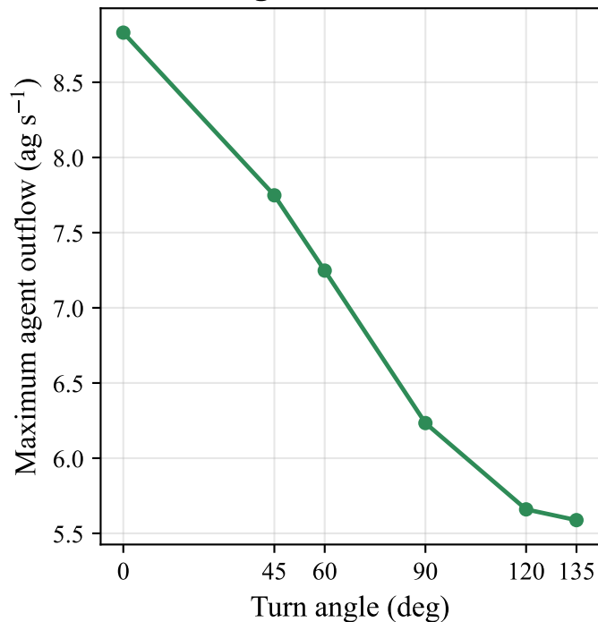
(b) Maximum agent outflow vs bend angle
