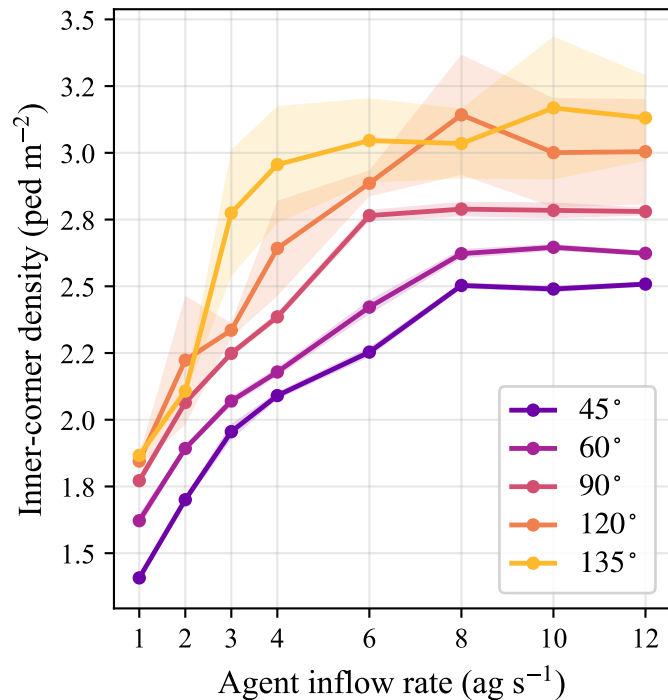
(c) Inner-corner density vs inflow rate
