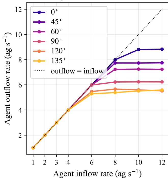
(a) Outflow rate at different bend angles
