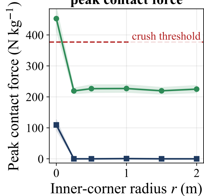
(a) Inner-corner peak contact force
