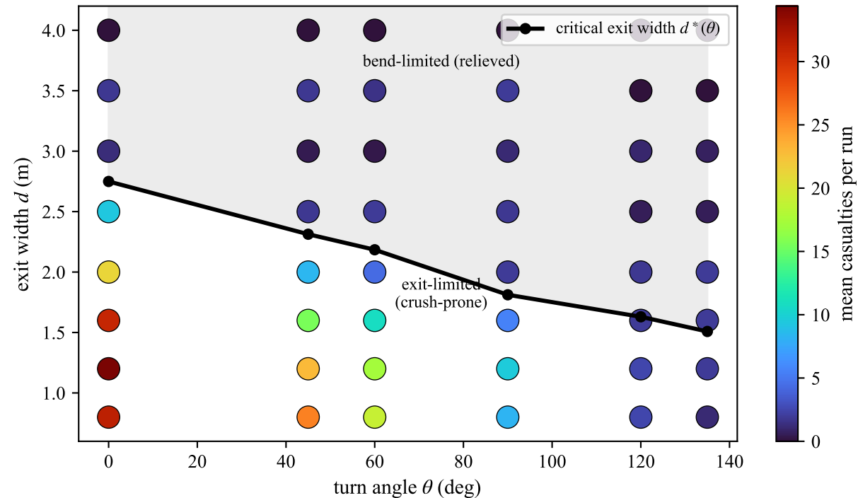
Crush across the turn-angle–exit-width plane
