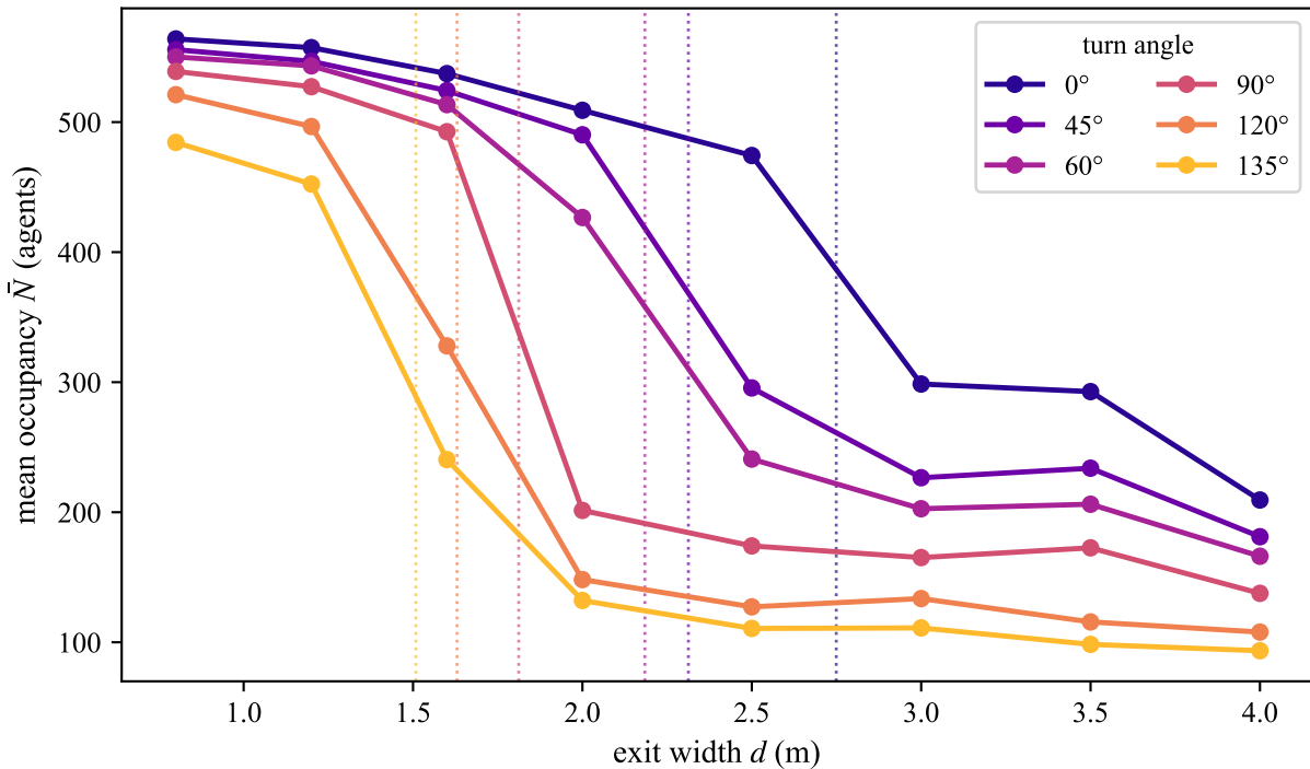
Occupancy transition versus exit width
