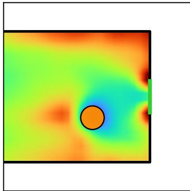
(b) single pillar, offset (2.2 m)
