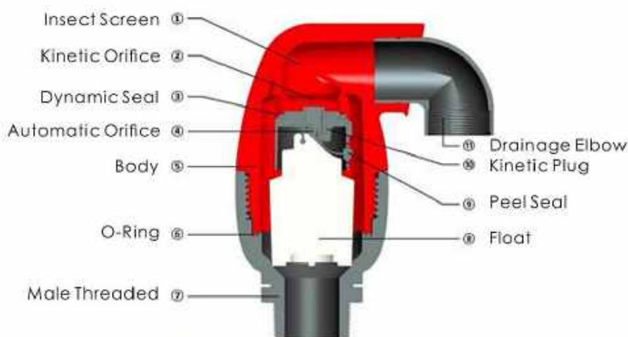
Air Relief and Intake (Pipeline Filling, Draining and Vacuum Conditions)
