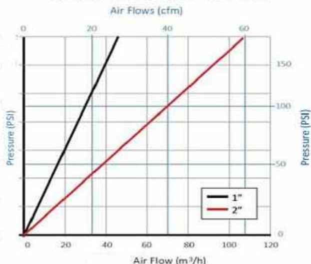
Air Release (Pressurized Operation)
