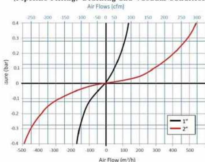
Air Relief and Intake (Pipeline Filling, Draining and Vacuum Conditions)
