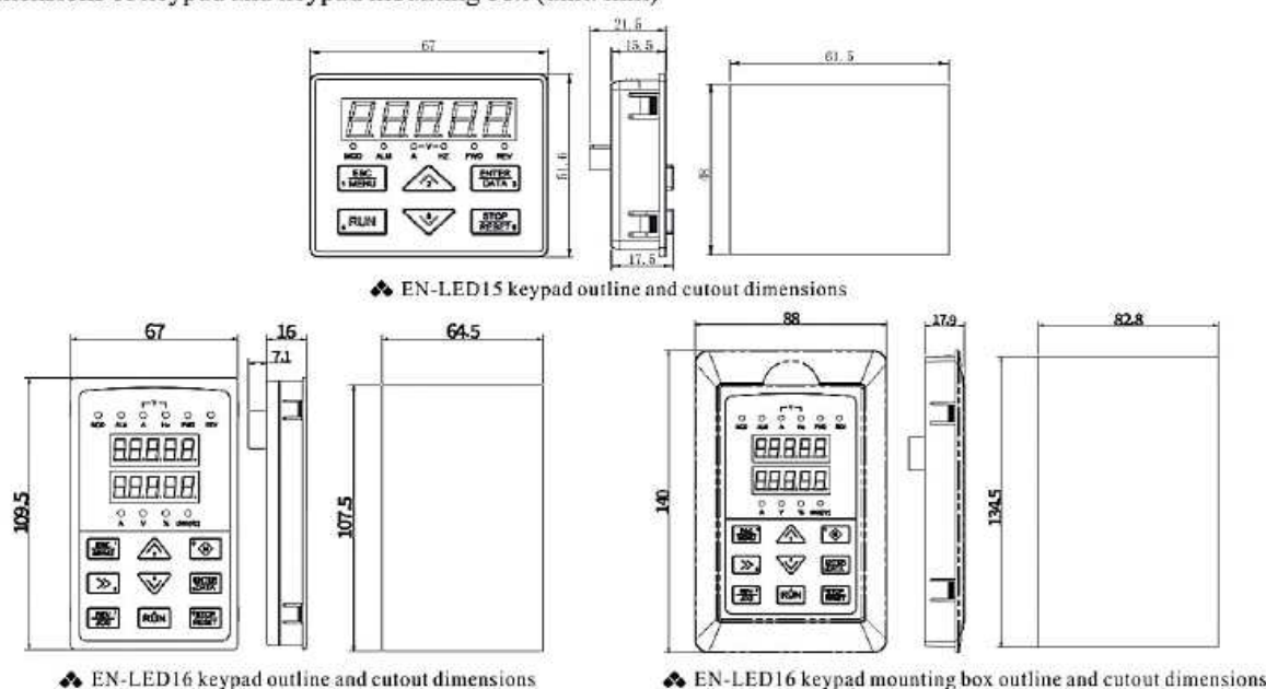
EN-LED16 keypad outline and cutout dimensions
