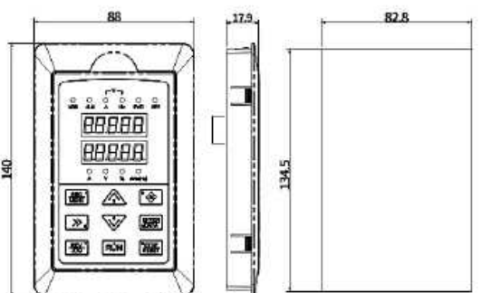
❖ EN-LED16 Keyboard Mounting Box Shape and Cutout Dimensions
