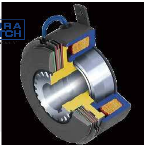
Electricmeganetic Clutch
