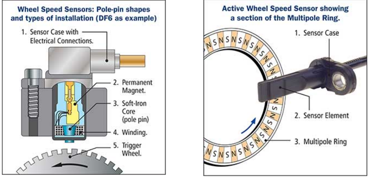
Figure 1.4: Passive (left) and active (right) wheel speed sensors from [6]
