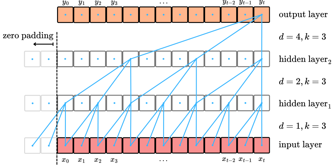
Figure 3.12: Dilated causal convolution
