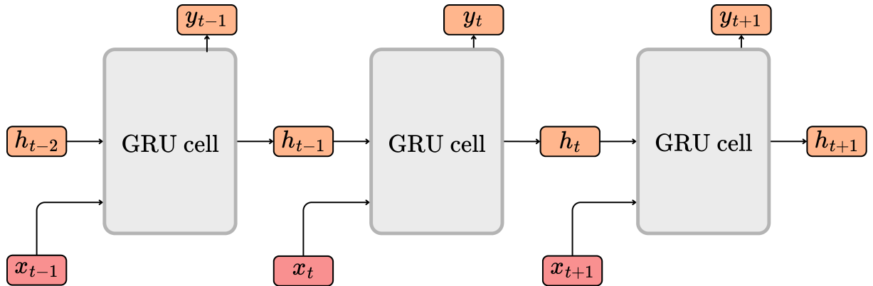
Figure 3.9: GRU sequence unfolded in time
