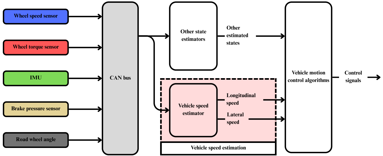
Figure 2.3: Vehicle speed estimation in the simplified control
