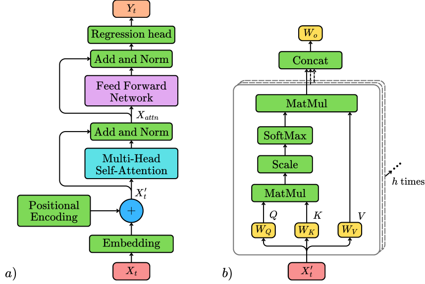
Figure 3.15: a) Transformer encoder block with regression head b) Multi-head self-attention mechanism
