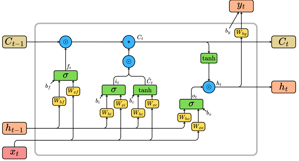
Figure 3.7: LSTM unit with the gating mechanisms
