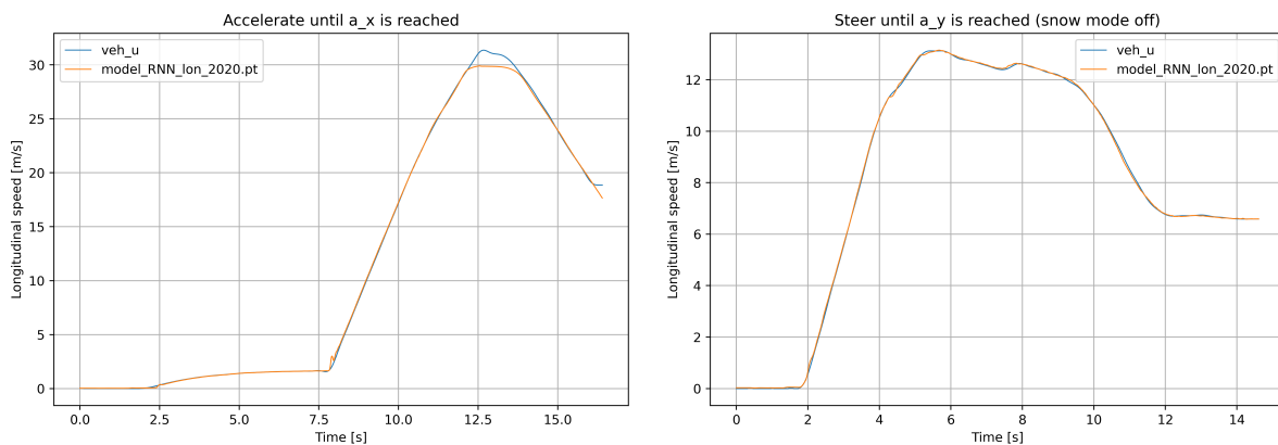
Figure 3.5: Predictions of the best performing RNN architecture on the validation dataset after finetuning (left: worst case, right: best case)
