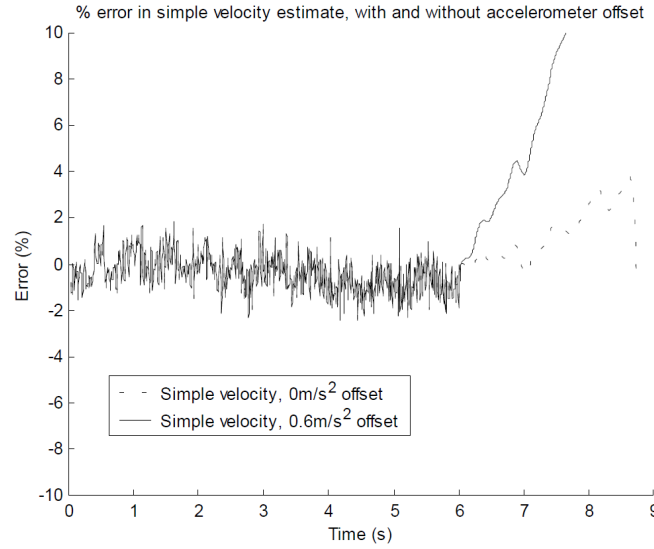
Figure 1.6: Simple algorithm for estimating vehicle speed form [10]
