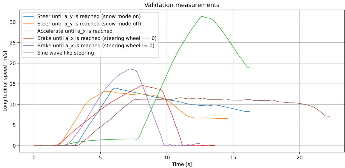
Figure 2.2: Recorded validation measurements for vehicle speed estimation
