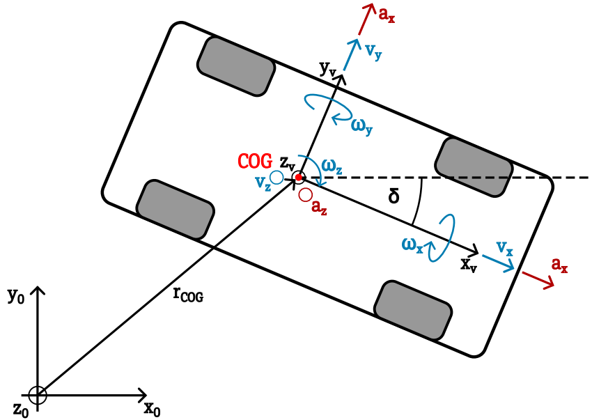
Figure 1.1: Vehicle speeds
