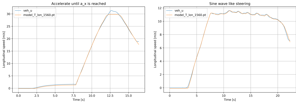
Figure 3.16: Predictions of the best performing transformer architecture on the validation dataset after finetuning (left: worst case, right: best case)
