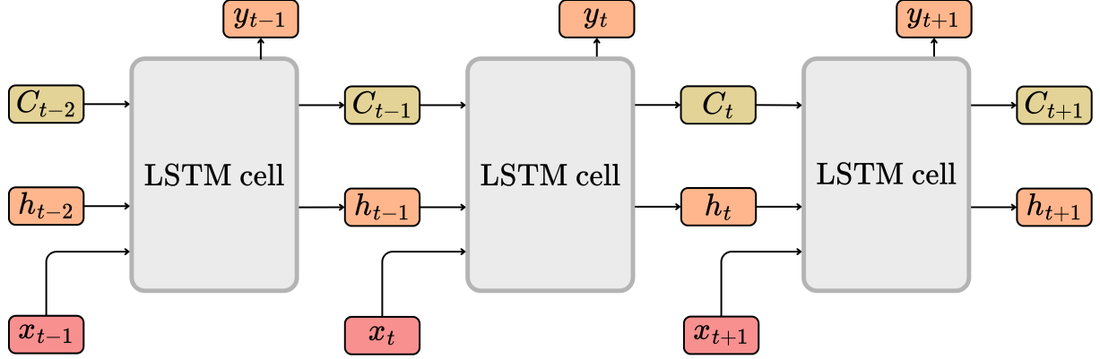
Figure 3.6: LSTM sequence unfolded in time
