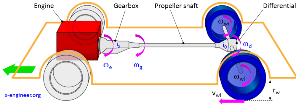
Figure 1.2: Calculating vehicle speed from engine speed [1]
