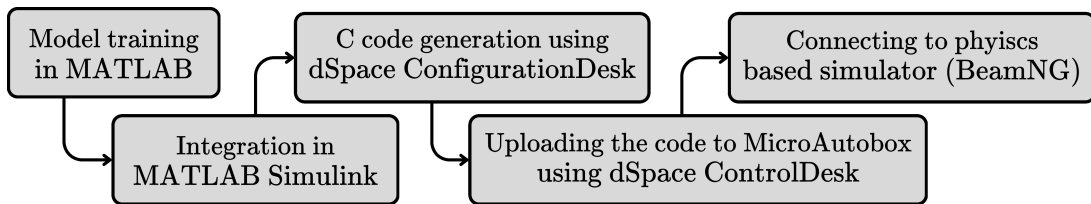
Figure 5.2: Toolchain of the real time implementation
