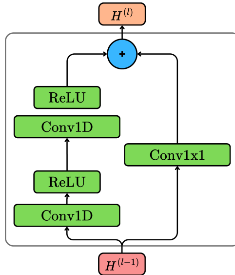
Figure 3.13: TCN residual block with two dilated causal convolutional layers
