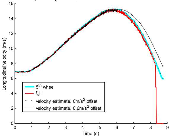
Simple velocity estimate, with and without accelerometer offset
