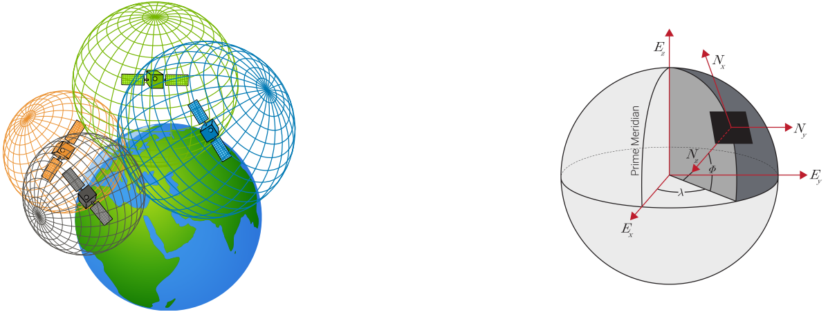
Figure 2.5: Trilateration (left) from [8] and ECEF coordinate system (right) from [9]
