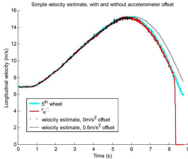
Figure 2.6: Simple algorithm for estimating vehicle speed from [11]
