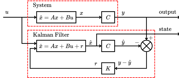
Figure 2.7: Vehicle speed estimation with Kalman filter from [12]
