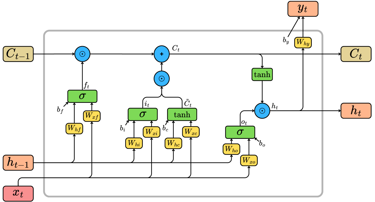
Figure 3.8: LSTM unit with the gating mechanisms
