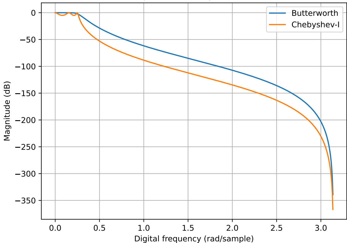
Response of Designed Filters
