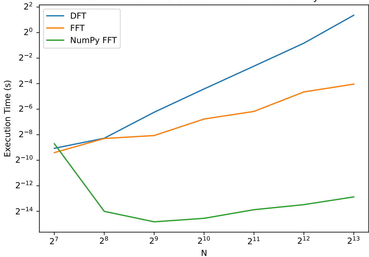
Execution Time Differences: DFT vs FFT vs NumPy FFT
