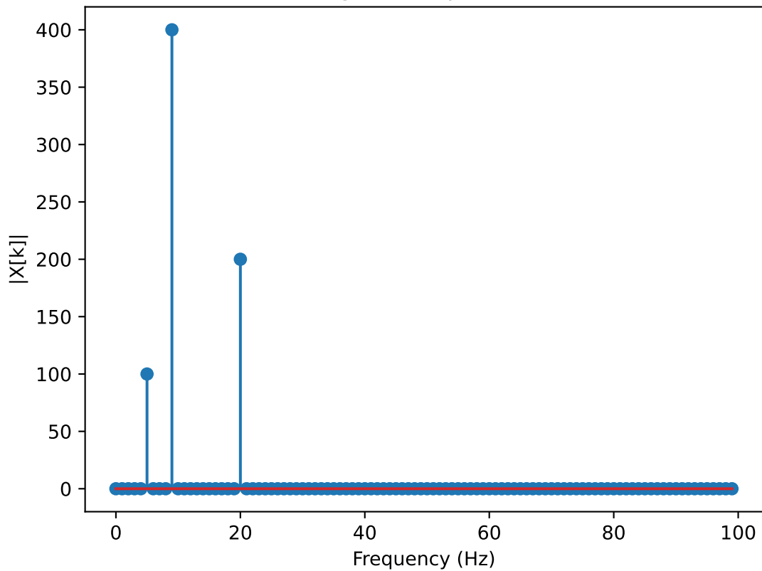
Magnitude Spectrum
