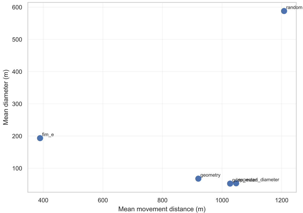
Movement–localization Pareto plane
