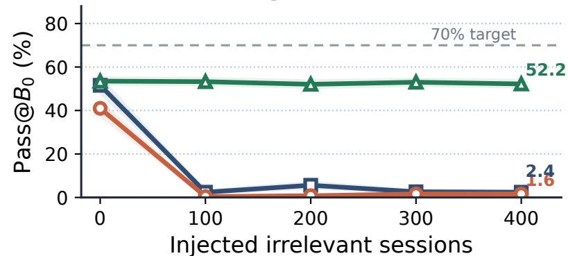
Qwen 8B
