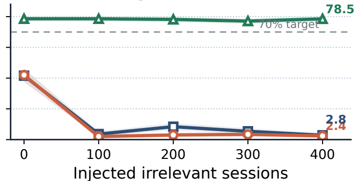
Qwen 32B
