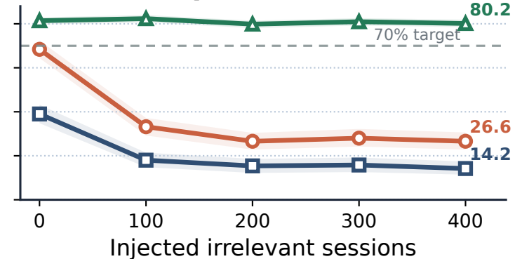
Qwen 235B
