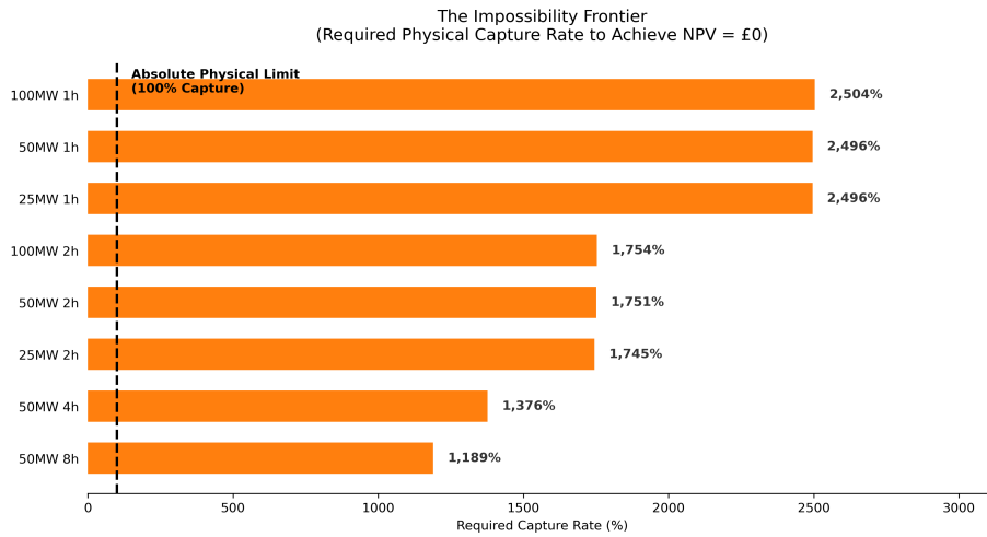
Figure 7 — The Impossibility Frontier (Conceptual). To achieve break-even on constraint revenue alone, exceeding the physically available constraint opportunity. This illustrates that the constraint opportunity is structurally insufficient.
