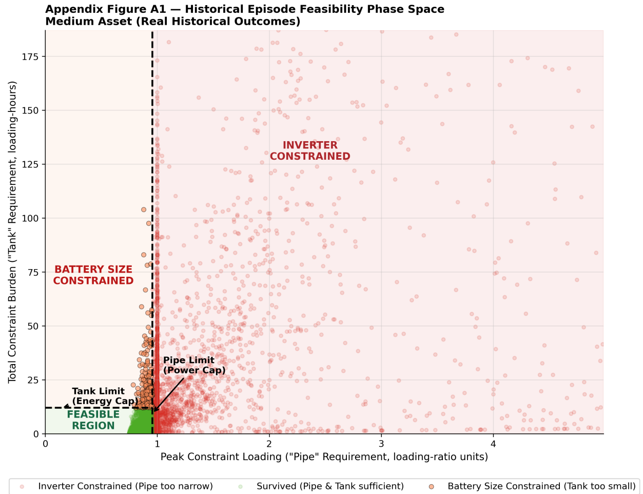
Figure 4: Figure 4 — The Feasibility Pipe & Tank Framework
