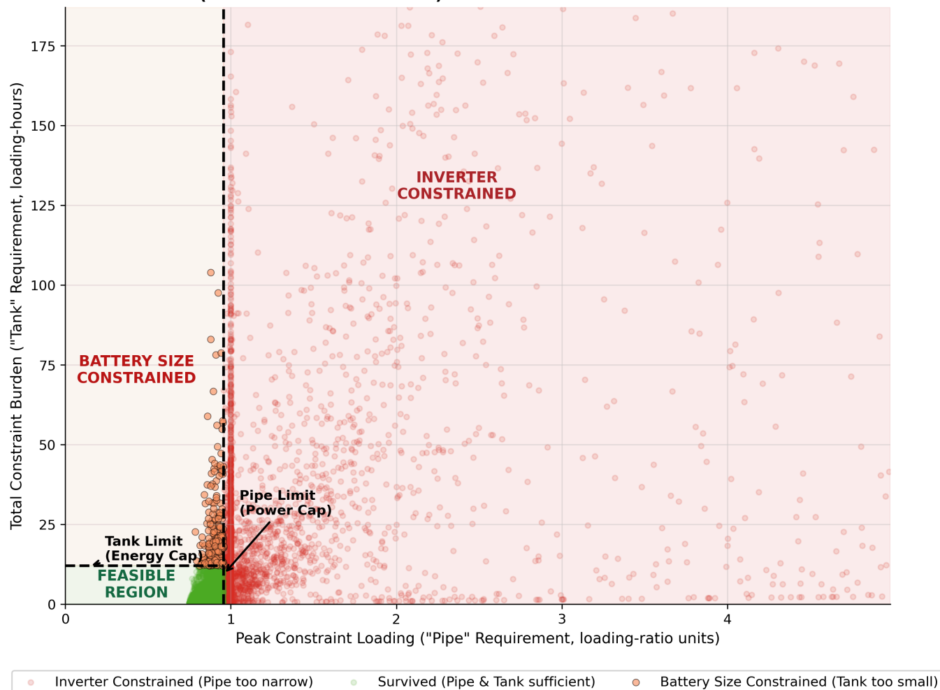
Appendix Figure A1 — Historical Episode Feasibility Phase Space Medium Asset (Real Historical Outcomes)
