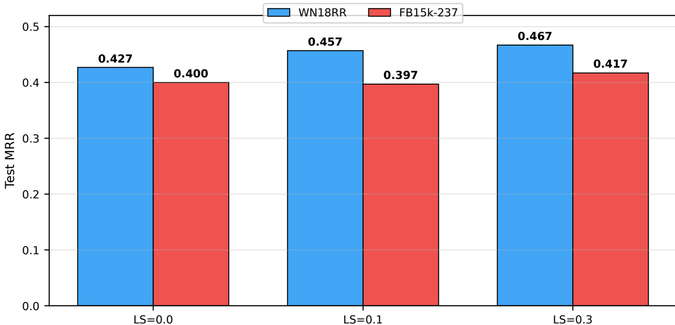
Label Smoothing Effect: Consistent Across Datasets
