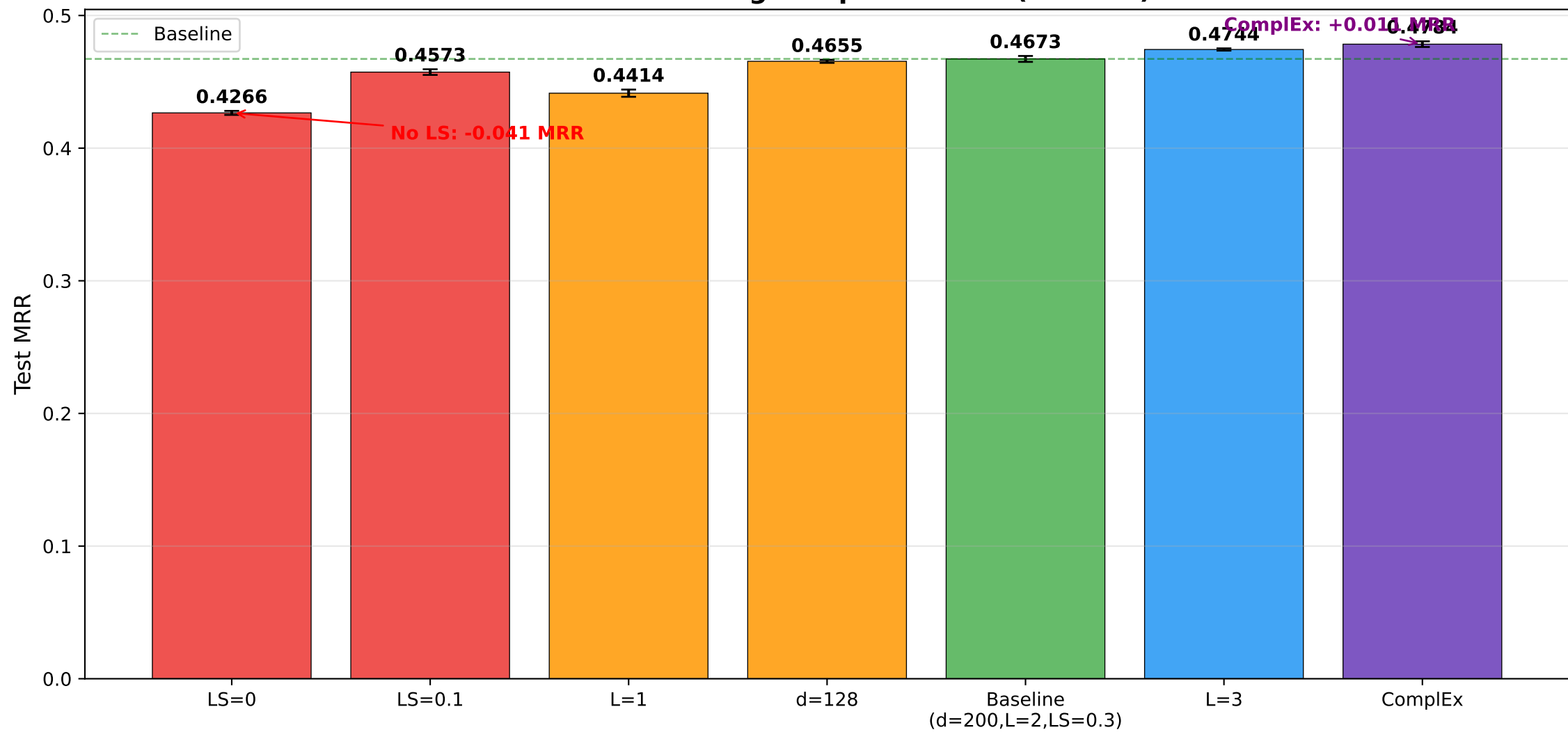
WN18RR: Training Recipe Ablation (3 seeds)
