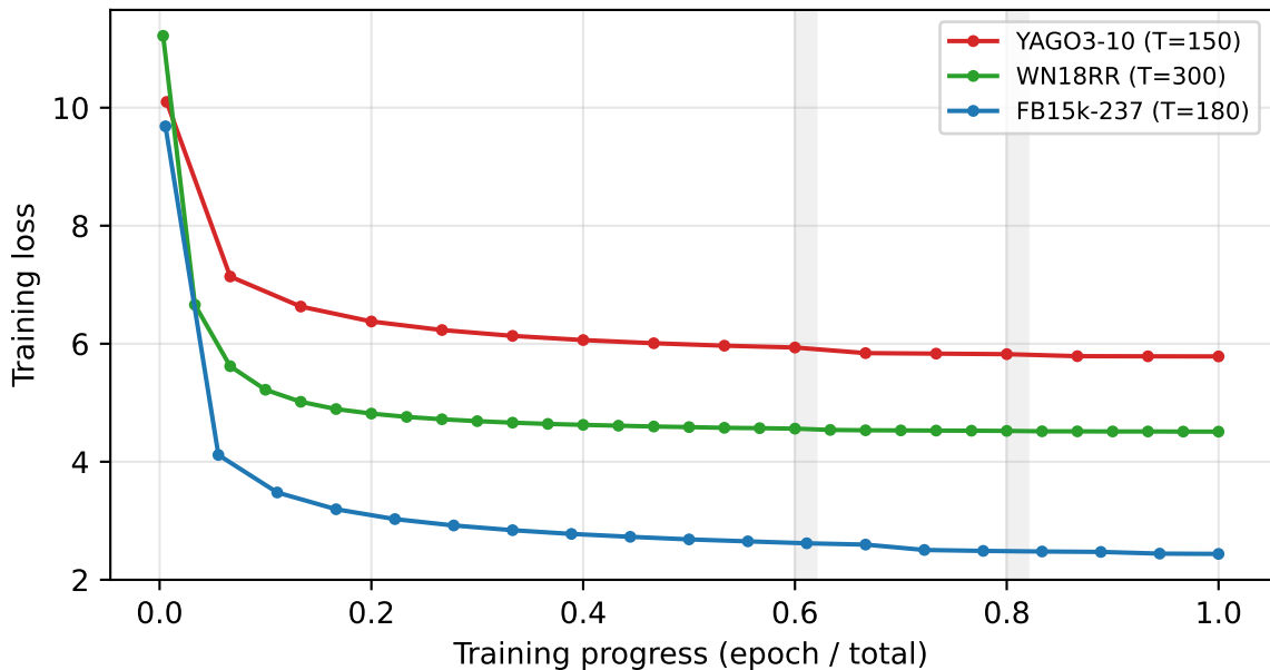
Training loss curves
