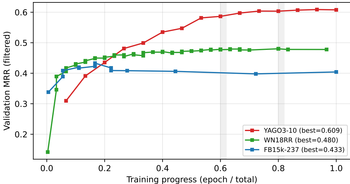
Validation MRR curves
